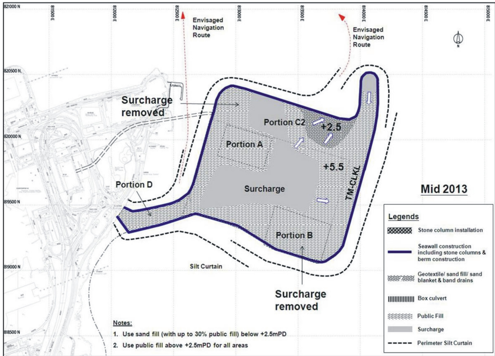
Figure 18 - Outline of Construction Sequence (Sheet 7 of 10)
